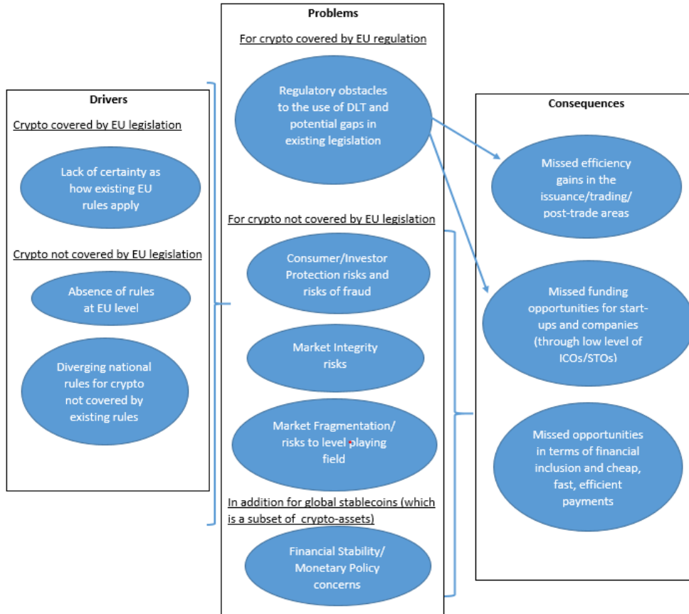
Figure 2: Problem tree
