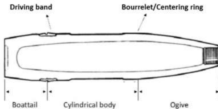
FIGURE 11: GENERIC ARTILLERY SHELL DESIGN
