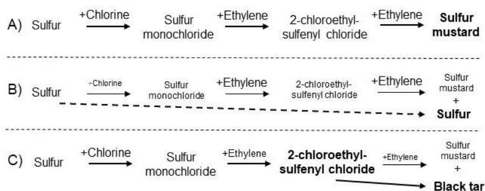
FIGURE 6: (A) THE LEVINSTEIN PRODUCTION METHOD FOR SULFUR MUSTARD; (B) SHORTAGE OF CHLORINE LEADS TO A FAILURE TO ACTIVATE MOST OF THE SULFUR ADDED. SULFUR BYPASSES THE PRODUCTION ROUTE AND REMAINS IN THE FORM OF A YELLOW POWDER; (C) SHORTAGE OF ETHYLENE GAS RESULTS IN THE PRESENCE OF BLACK TAR.
